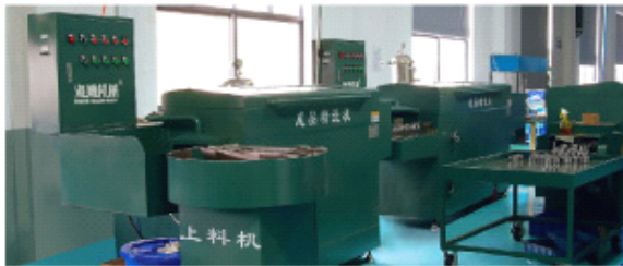
Automatic oil stamping machine CNC Heat Treatment Vertical Broaching Laser marking machine Wire mesh conveyor belt Cleaning machine
